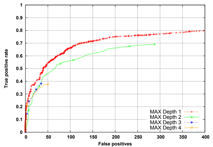
Fig. 8. Variation of the maximum depth parameter (Maximum depth per weak learner) values for the MB-LBP features based classifiers.
