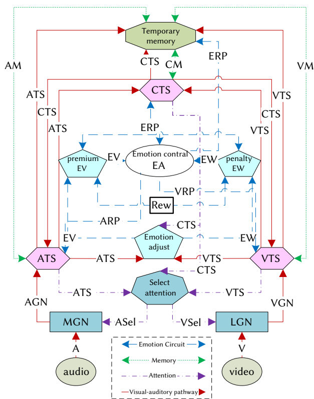
Fig. 18. Cognitive architecture of media computing.
