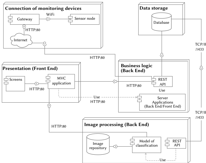
Fig. 7. Component diagram.
