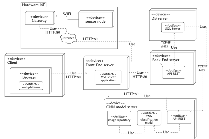
Fig. 8. Deployment diagram.
