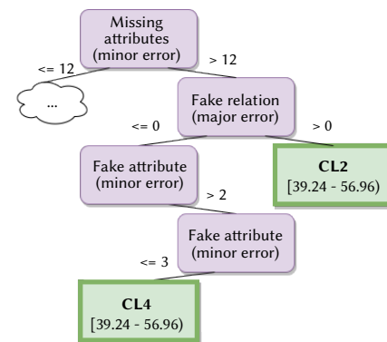
Fig. 7. Decision tree. In-game outcomes for less successful students based on in-game errors (CL2 and CL4).
