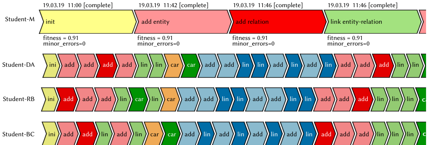
Fig. 12. Traces of students who obtained a fitness &gt; 0.90.
