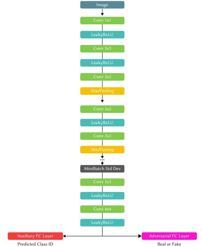
Fig. 4: Discriminator of the Style-based Generative Adversarial network with an auxiliary output block for tumor classification.
