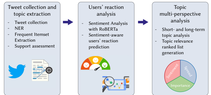
Fig. 2. Architecture pipeline.
