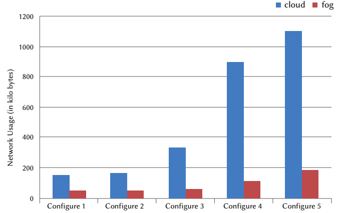
Fig. 6. Fog computing and cloud computing comparison for Network Usage.
