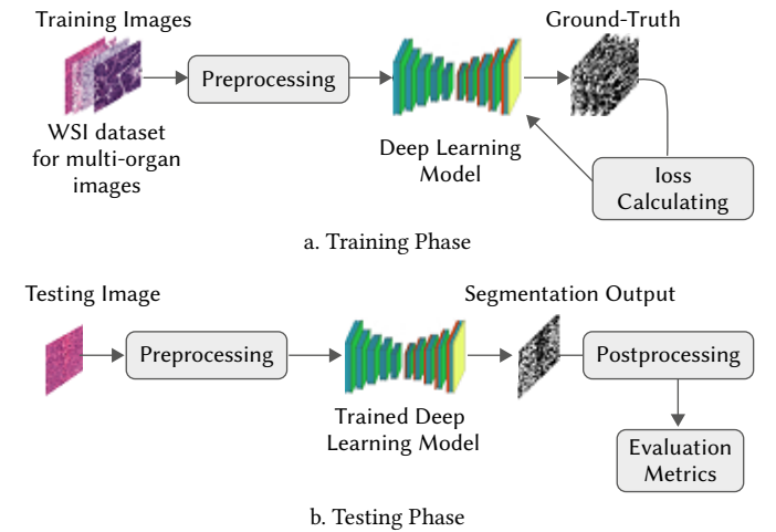
Fig. 2. Nuclei segmentation framework: a) training phase, and b) testing phase.
