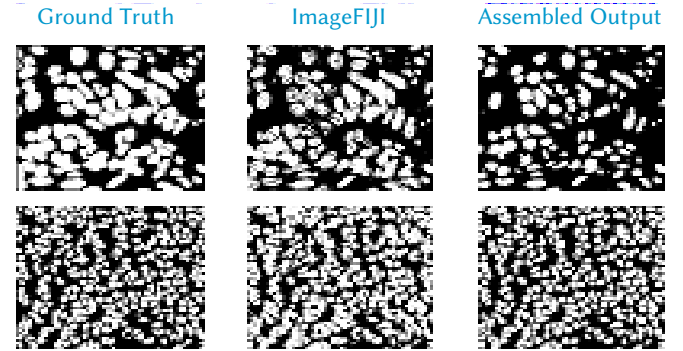
Fig. 12. Segmentation results of (middle) ImageJ software, and (right) ensemble of U-Net, PSPSegNet, and Self-Correction models.
